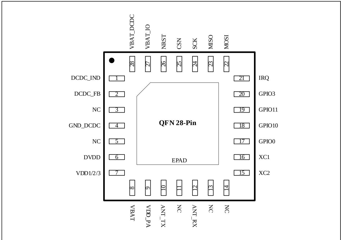
Figure 4-1 Pin diagram
